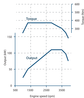
4P10-KAT4 110 kW/3,500 RPM 370 Nm/1,320 - 2,840 RPM
